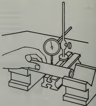
FIGURE 10-7. Checking a piston pin for bends.
